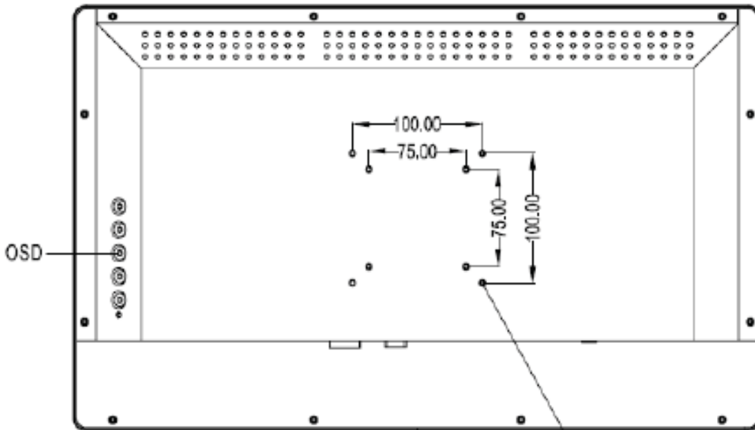
Back View
